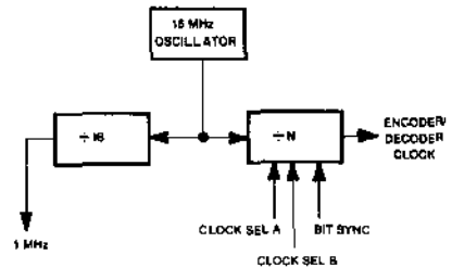
Fig. 2-11. Block diagram of the timing circuit.
